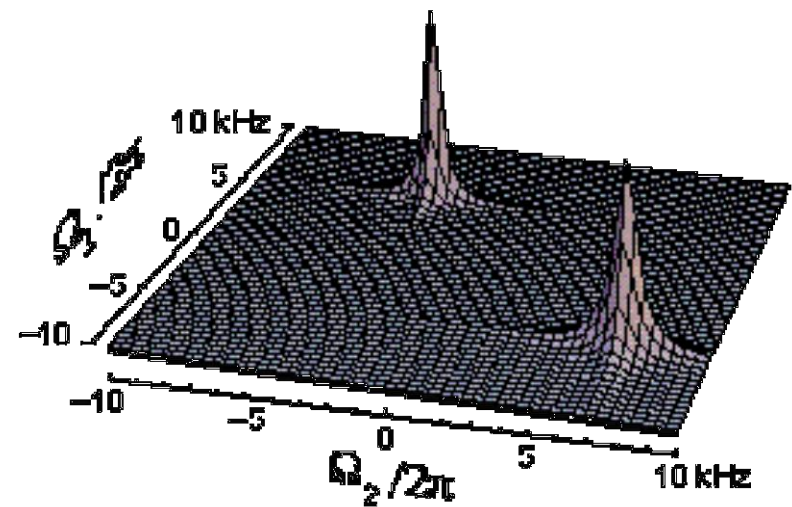
'States' spectrum
